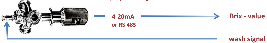
Sensor connection with spray cleaning
